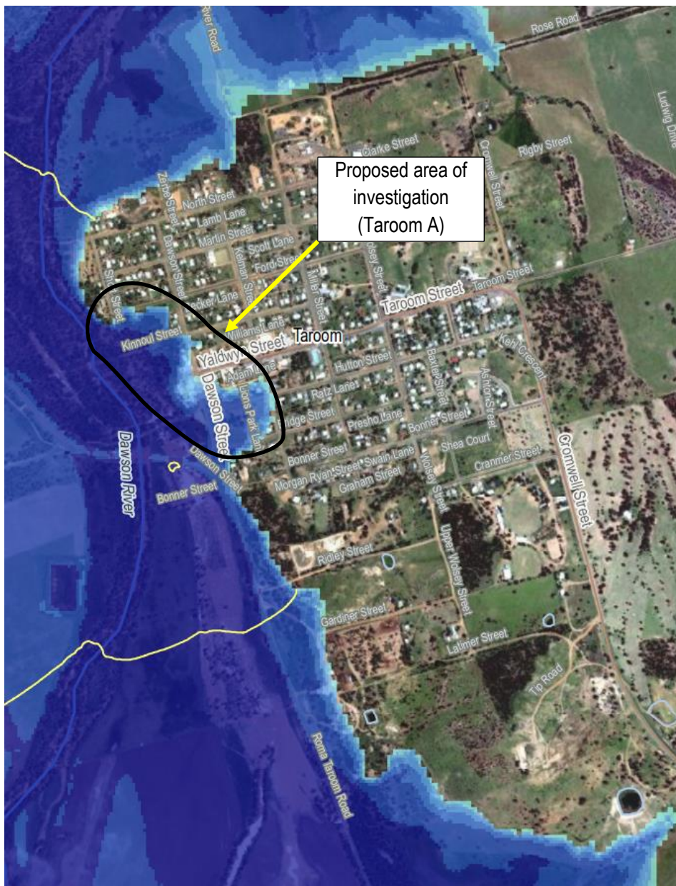
Image: Proposed area of investigation with 1% + CC AEP flood inundation depths shown
