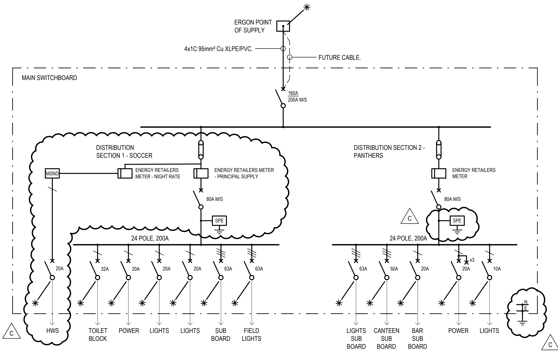
SINGLE LINE DIAGRAM
