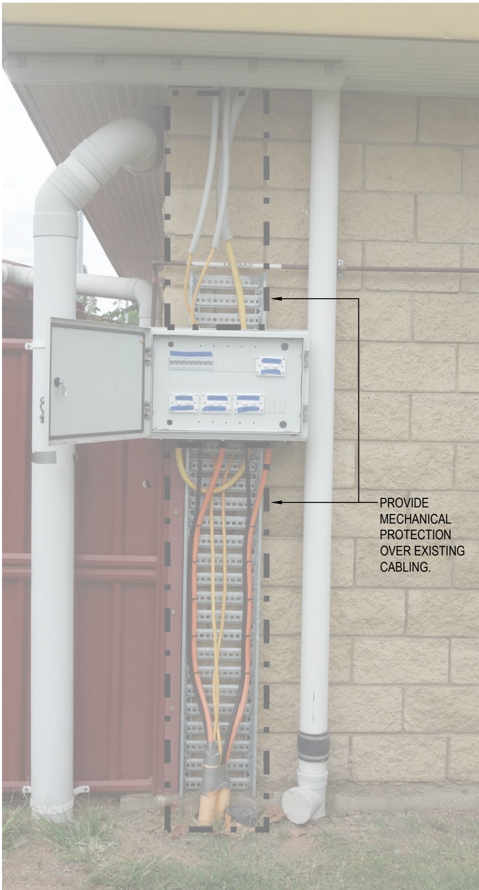
EXISTING CONTROL PANEL
